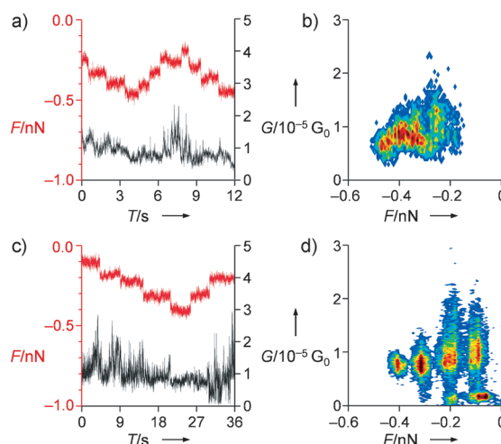
Figure 4. Conductance response as a function of applied force for a,b) \text{HS}(\text{CH}_2)_8\text{SH} and c,d) \text{Ph}_2\text{P}(\text{CH}_2)_8\text{PPh}_2 . To avoid complications to the data from stochastic changes in S-Au contact geometries, the presented traces are limited to those around 1 \times 10^{-5} G_0 .
